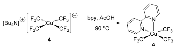
Scheme 3. Synthesis of [(bpy)Cu(CF 3 ) 3 ] ( 6 ) from [Bu 4 N] + [Cu(CF 3 ) 4 ] − ( 4 ).
